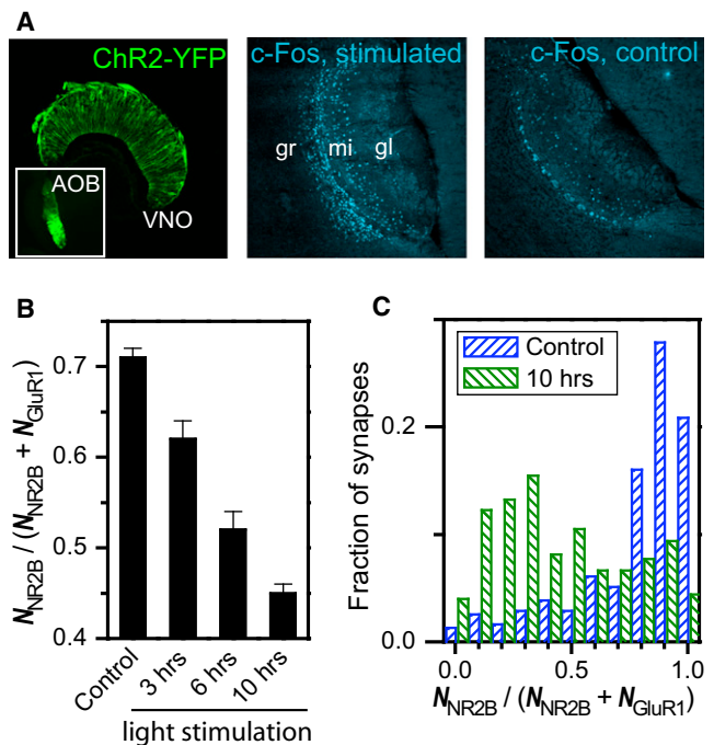
Figure 7. Changes in the Receptor Composition of AOB Synapses in Response to VNO Stimulation
