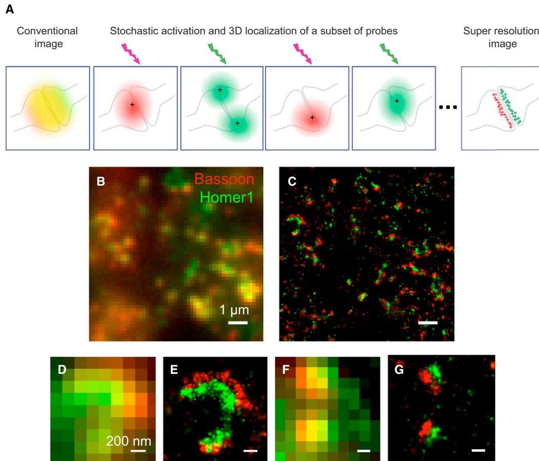
Figure 1. STORM Imaging of Pre- and Postsynaptic Scaffolding Proteins
