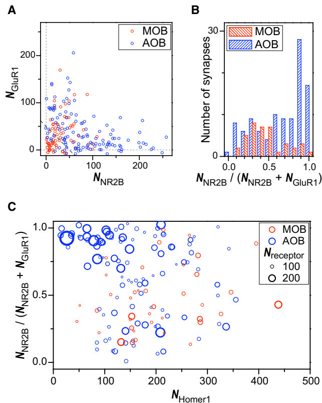
Figure 6. Composition of Glutamate Neurotransmitter Receptors at Synapses
