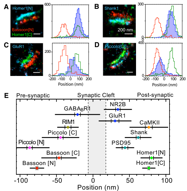
Figure 4. Axial Positions of Synaptic Proteins
