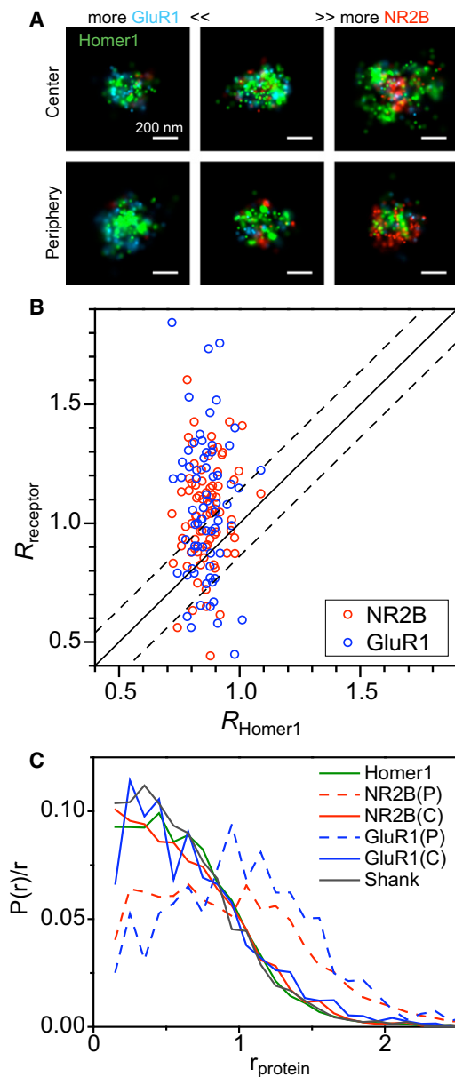
Figure 5. Radial (Lateral) Distribution of Glutamate Neurotransmitter Receptors at Synapses
