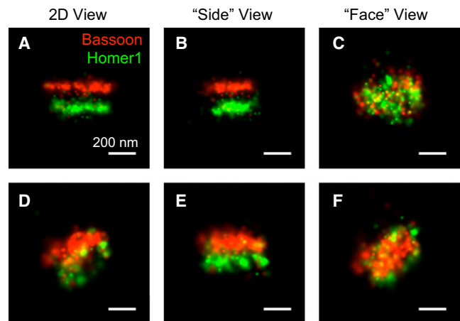
Figure 2. 3D STORM Images of Synapses
